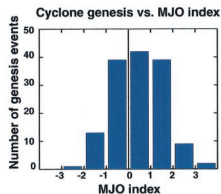
Fig. 3. Histogram of tropical cyclone genesis events for the western Atlantic, Caribbean Sea, and Gulf of Mexico to the west of 77.5^\circ\text{W} as a function of the MJO index. Histogram categories are each 1 SD of the MJO index.
