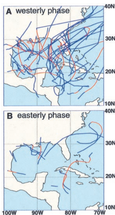
Fig. 2. Tracks of Gulf of Mexico, Caribbean Sea, and western Atlantic tropical cyclones that form to the west of 77.5^\circ\text{W} when the MJO index has a magnitude greater than 1 SD from zero. Westerly (greater than 1 SD) (A) and easterly (less than -1 SD) (B) phases are displayed. Tropical storm tracks [winds between 34 and 64 knots ( 17 to 33 \text{ m s}^{-1} )] are plotted in blue. Hurricane tracks [winds greater than 64 knots ( 33 \text{ m s}^{-1} )] are plotted in red. Cyclone data span the period 1949–1997.
